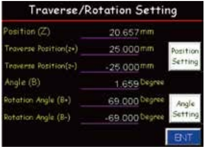
▲ Traverse/Rotation setting
